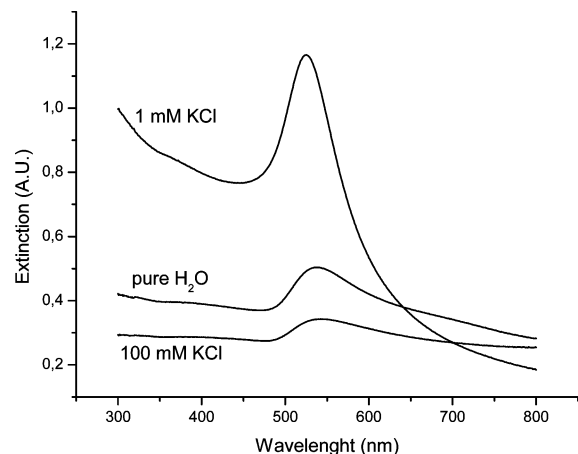
Figure 2. Absorption spectra of gold colloids produced by laser ablation in different aqueous solutions.
