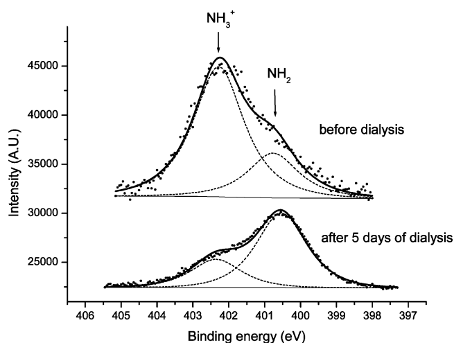
Figure 8. High-resolution XPS spectra of the nitrogen (N1s) peak of gold nanoparticles produced by laser ablation in a 10 mM aqueous solution of propylamine. The upper figure is an as-produced sample, while the lower one was dialyzed for 5 days prior to measurement.
