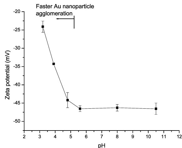
Figure 7. \zeta potential of gold nanoparticles produced in 10 mM aqueous NaCl solutions at different pH values.
