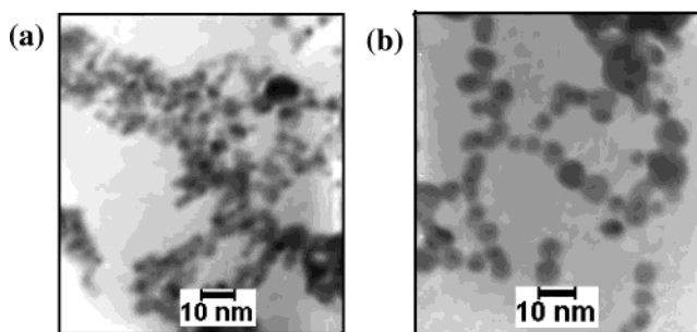
Figure 6. TEM micrographs of gold particles prepared by the femtosecond laser ablation of gold in (a) 10 mM NaCl and (b) NaOH (pH 9.4).
