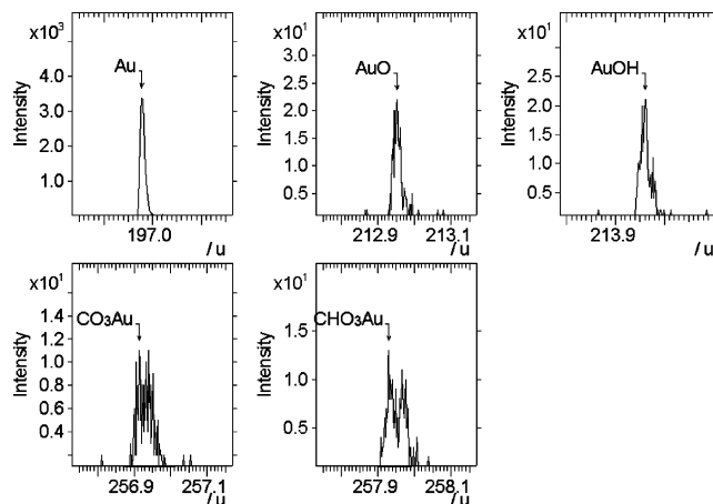
Figure 5. Negative TOF-SIMS spectra for mass regions corresponding to \text{Au}^- , \text{AuO}^- , \text{AuOH}^- , \text{CO}_3\text{Au}^- , and \text{CHO}_3\text{Au}^- . Particles were prepared in deionized water.
