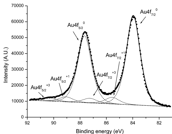
Figure 3. High-resolution Au4f XPS spectrum of Au nanoparticles produced by laser ablation in deionized water.
