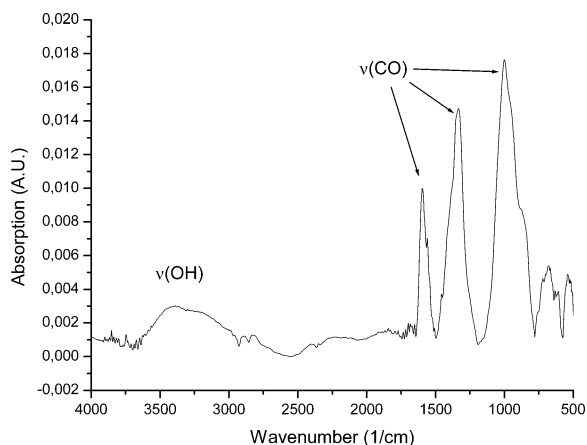
Figure 4. FT-IR spectra of gold nanoparticles produced in deionized water.
